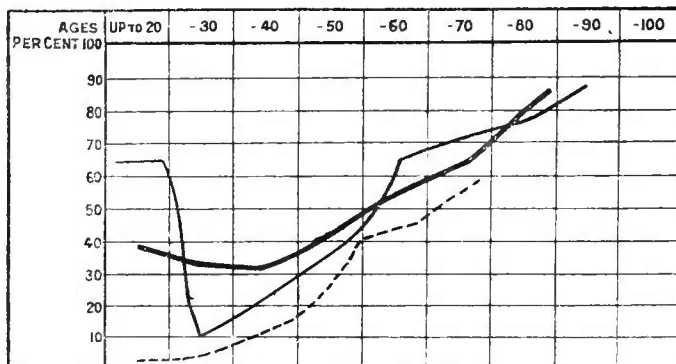
The dotted line shows the frequency of granular kidney in proportion to healthy kidneys, derived from Mahomed's figures.
