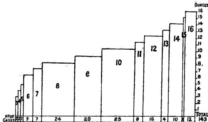
Diagram in which the weights in ounces of the two kidneys together are shown by the height of the vertical line, while the number of cases in which the kidneys were of the given weight is shown by the length of the base line.
