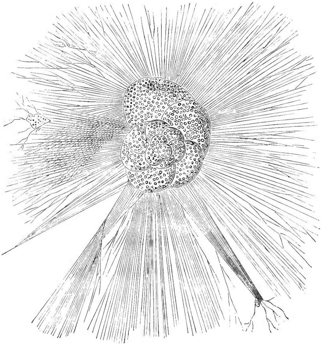
Fig. 120. — Discobina globularis .
